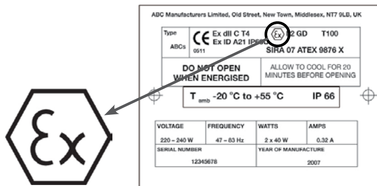
Figure 1 Typical ATEX equipment marking plate
